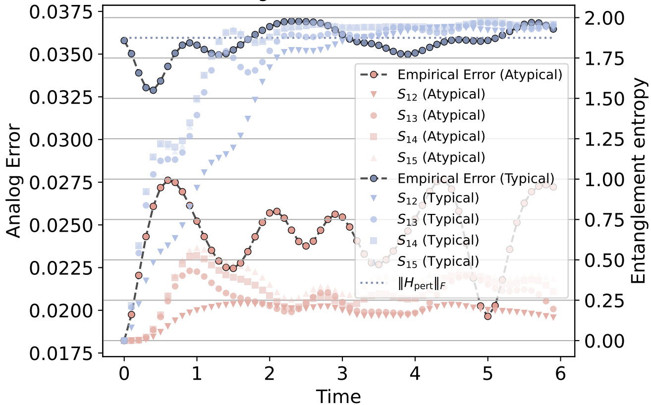
TFIM, one segment evolution with disorder
